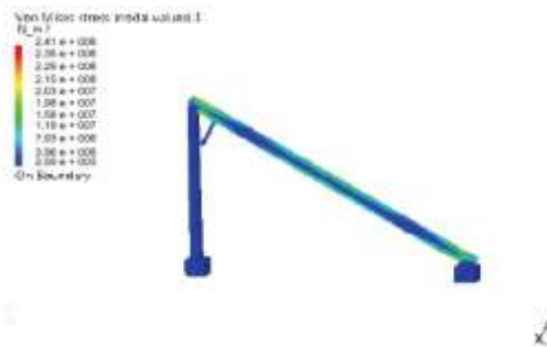
Fig. 5.2 General Von Mises maximum and minimum stress
